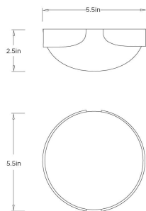
DFC30 ELARA FLUSH MOUNT
