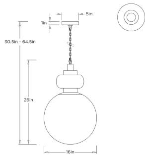
*ADDITIONAL CHAIN AVAILABLE DSC12 ROSEMONT LARGE PENDANT A R T E R I O R S
