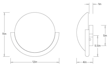
DWC101 ALICIA WALL SCONCE
