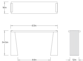
FLS13 ANTONINE CONSOLE
