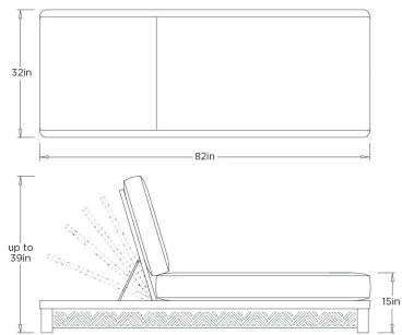
FTS04 EMOTO OUTDOOR CHAISE
